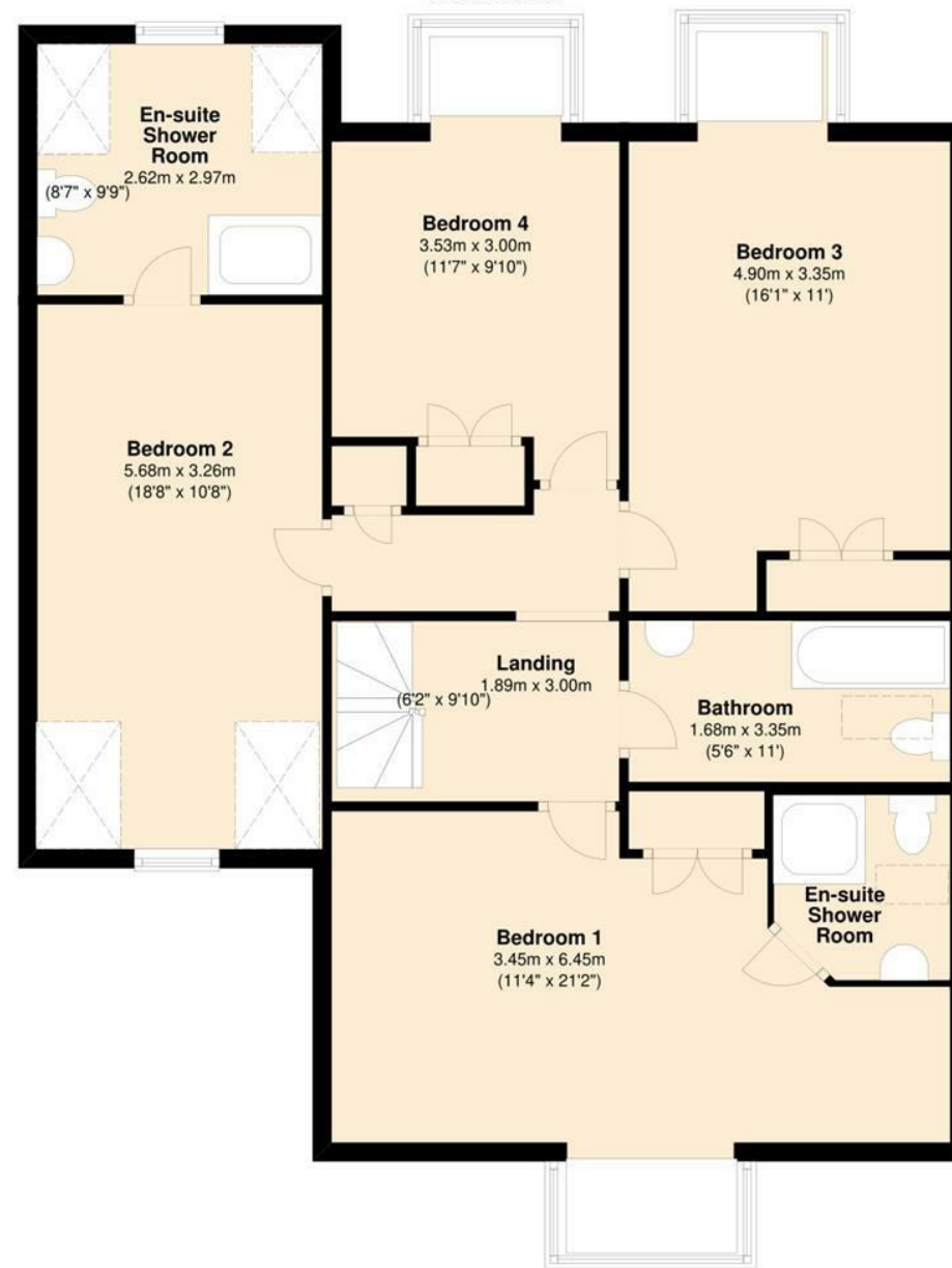
First Floor
